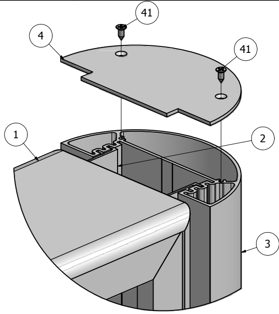
DETAIL A
